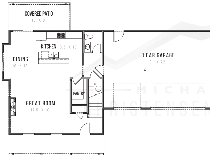
MAIN FLOOR
